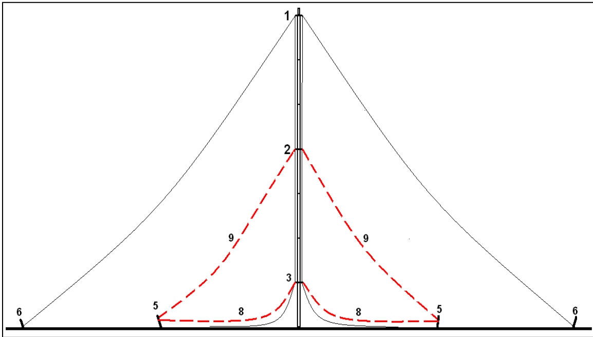
Figure 6. Installing the 28 ft (8.53 m) rope and preparing wires and ropes loose to lift the seven sections of mast to insert the eighth.
