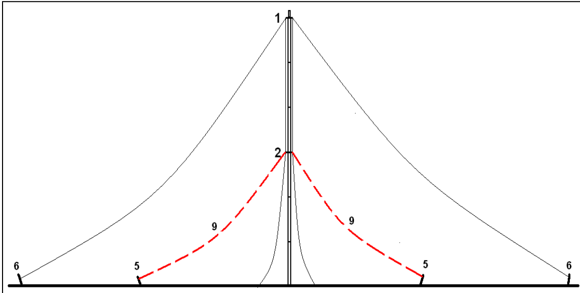
Figure 4. Securing the six sections of mast using the loops wires and rope loosely.
